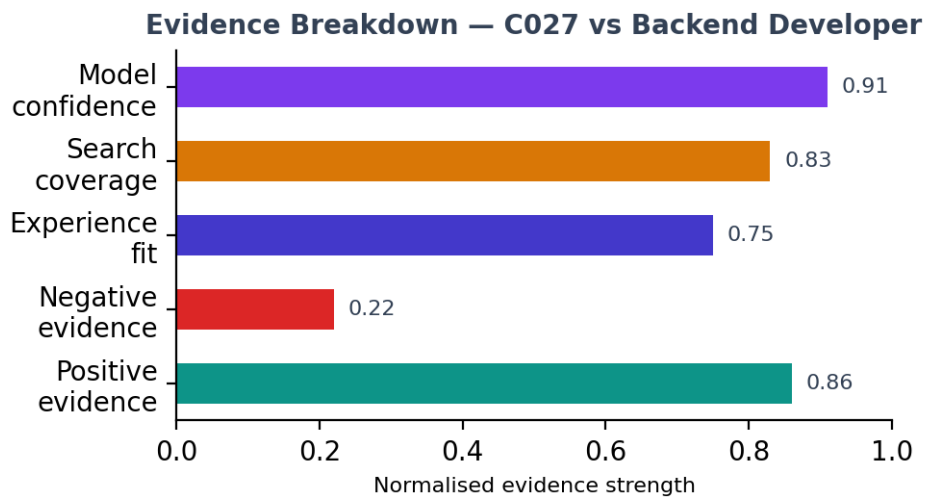
Figure 4. Component-level explanation for a sample candidate-job pair (C027 vs Backend Developer).
